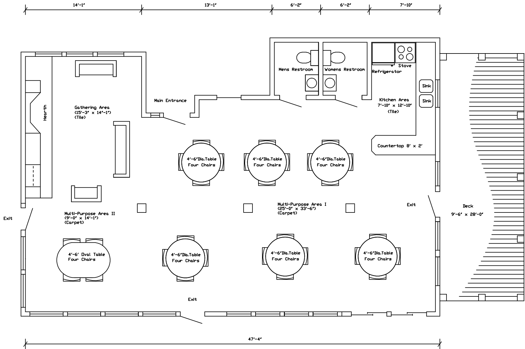
Kalb Gathering House Interior Plan
